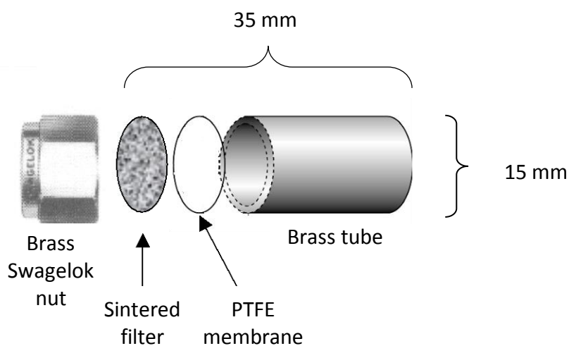
Figure M18.2. Permeation tube
